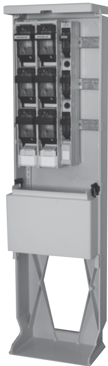
EHFERB/35 with disconnects fitted
